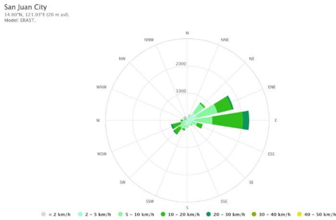
Figure 8 Windrose diagram of San Juan City, Philippines. Note. Adapted from Weather maps and forecast data, by Meteoblue, n.d. ( https://www.meteoblue.com/ ). Copyright [2026] by Meteoblue.
