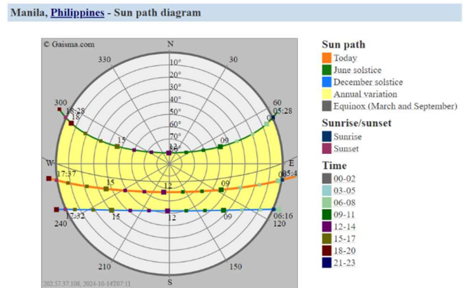
Figure 7 Manila, Philippines Sun Path Diagram. Note. Adapted from Sunrise, sunset, dawn and dusk times around the world , by Gaisma, n.d. ( https://www.gaisma.com/en/ ). In the public domain.
