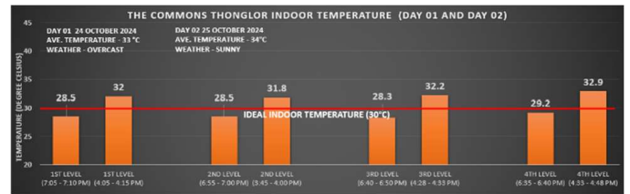
Figure 59 Indoor temperature for Day 01 and 02 of The Commons Thonglor.
