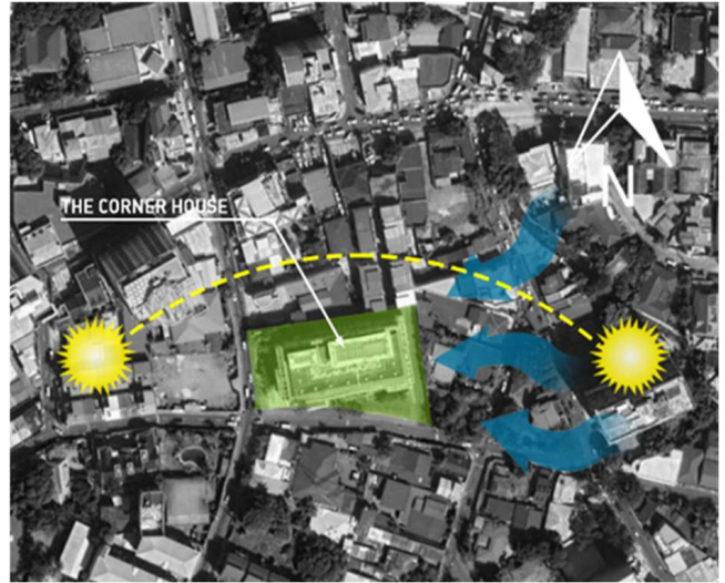
Figure 14 Position and orientation of the building mass. Note. Annotated image [Google Earth view of Bangkok, Thailand]. (n.d.). ( https://earth.google.com/web/ ). Copyright 2026 by Google.
