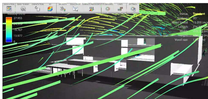
Figure 72 Airflow simulation along CM Recto Street illustrates the wind flow from the south direction.
