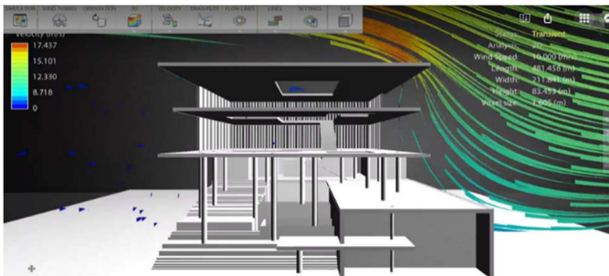
Figure 74 Airflow simulation showing the wind from the west direction.
